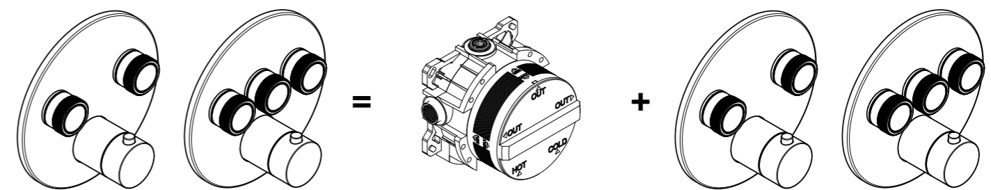
Termostatico incasso con deviatore Thermostatic mixer for concealed installation 2 vie | 2-way 3 vie | 3-way
